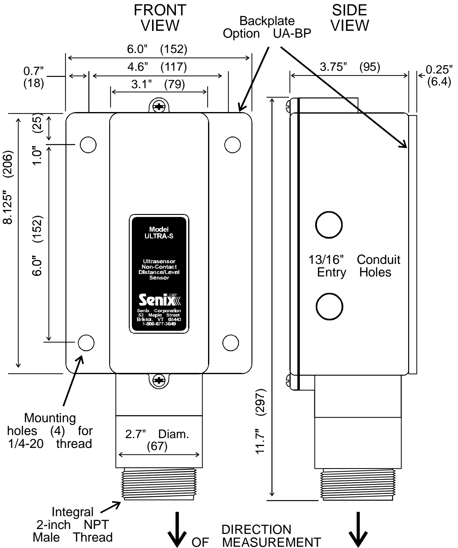
Model ULTRA-S and ULTRA-S-BP Dimensions
